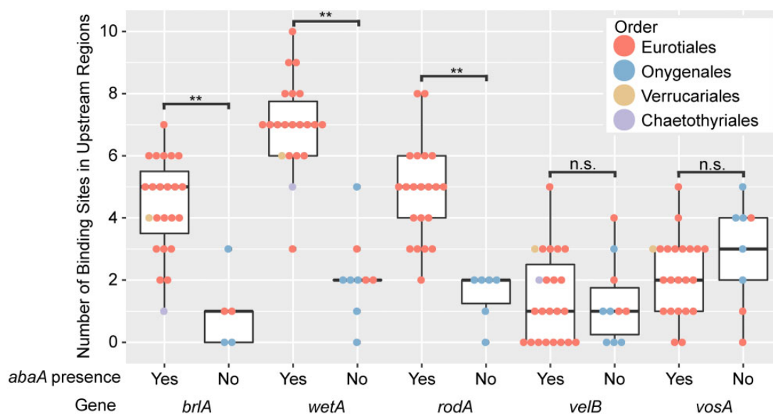
FIG. 3. —Species that lack abaA have fewer AbaA binding sites upstream of the protein-coding regions of many orthologous genes that are directly regulated by AbaA in Aspergillus nidulans . Box plot comparing the number of AbaA binding sites in the 1.5-kb upstream regions of the AbaA target orthologs for species with the abaA gene and species without the abaA gene (only species in Eurotiomycetes are shown in supplementary table S3, Supplementary Material online). ** P < 0.01 , n.s., not significant.
